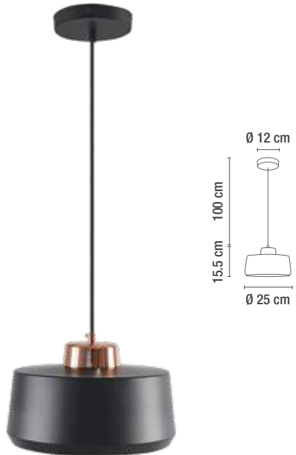
C219/NE
