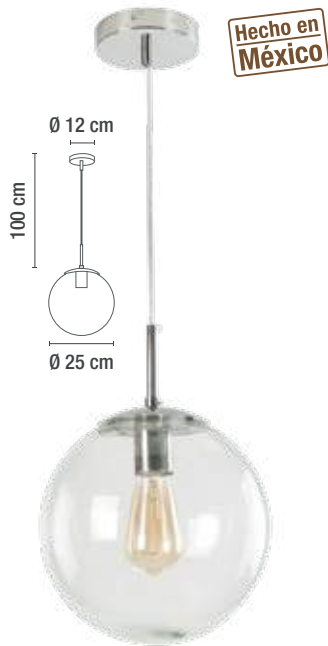
C110-R10/CR
