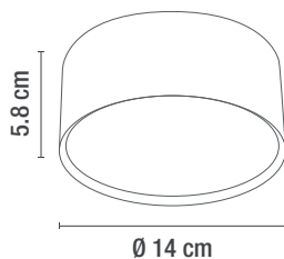
DLP098LED-F/BL
